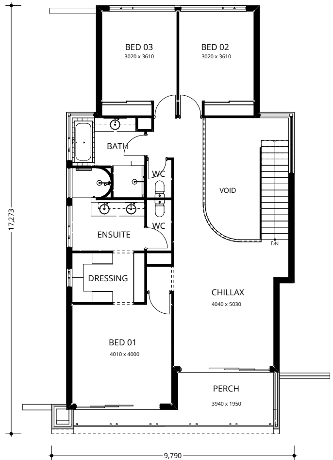
UPPER FLOOR
